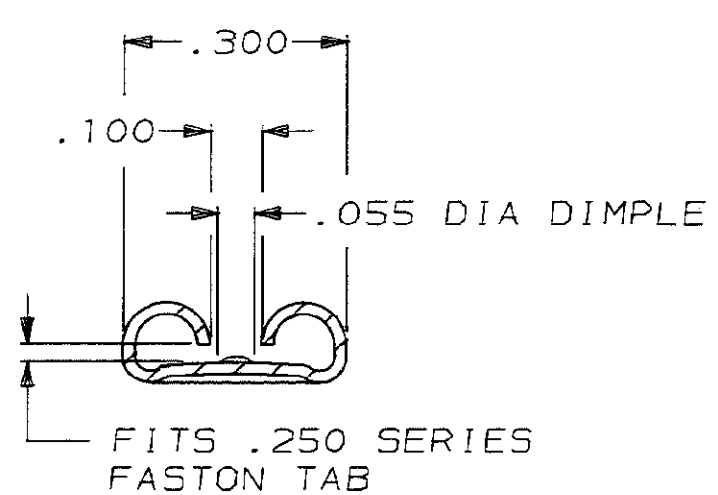
SECTION X-X
